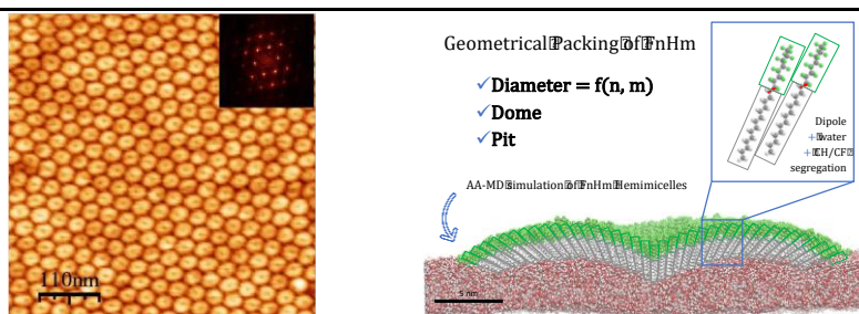
Figure: left: AFM image of a F8H18 monolayer on a silicon wafer. right: Scheme depicting the geometrical packing of the F n H m molecules within the hemimicelles, obtained from molecular dynamics simulations.
